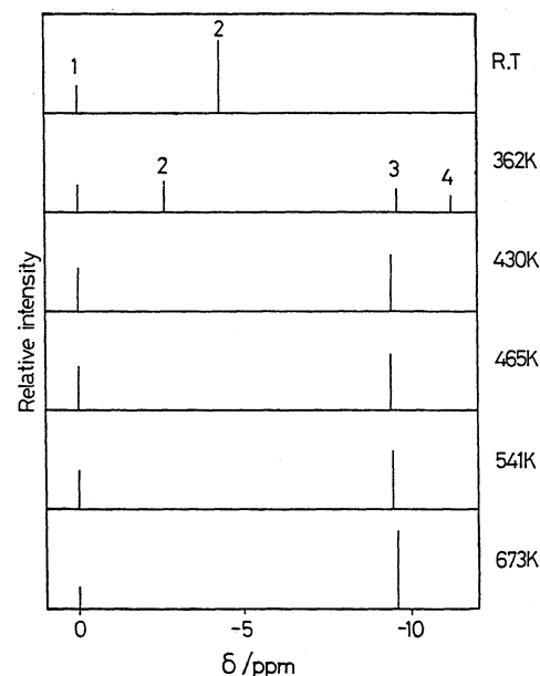
Fig. 3. ^{31}\text{P} NMR spectra of the thermal products of \text{CaCAP} \cdot 1.5\text{H}_2\text{O} . 1: Orthophosphate, 2: carbamoylphosphate, 3: diphosphate, 4: end \text{PO}_4 group of intermediate polyphosphate ( n > 3 ).
